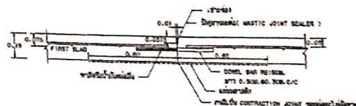
REINFORCED CONSTRUCTION JOINT AND CONTRACTION JOINT
